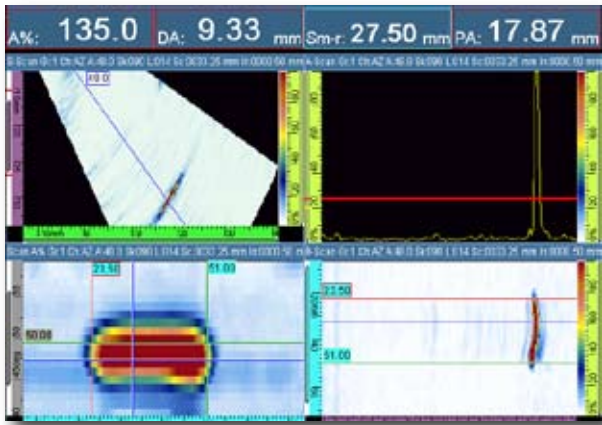
Results showing incomplete root penetration.
