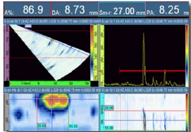
Results showing a crack in the root of the weld.
