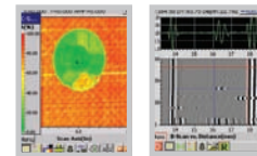
Far Left: Complete C-Scan Left: TOFD
