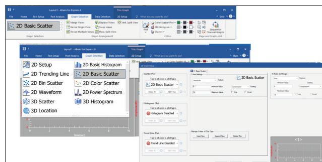
Figure showing the Graph Selection ribbon interface, the different available 2D plot options and an example of the new graph setup menu. The new menu is designed for easier plot definition.
