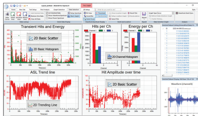
Example of single tab page showing several different types of 2D plots. Clockwise: Scattered and histogram combined plot, bar cumulative plots, line displays, waveform display, scattered plot and trend line plot.
